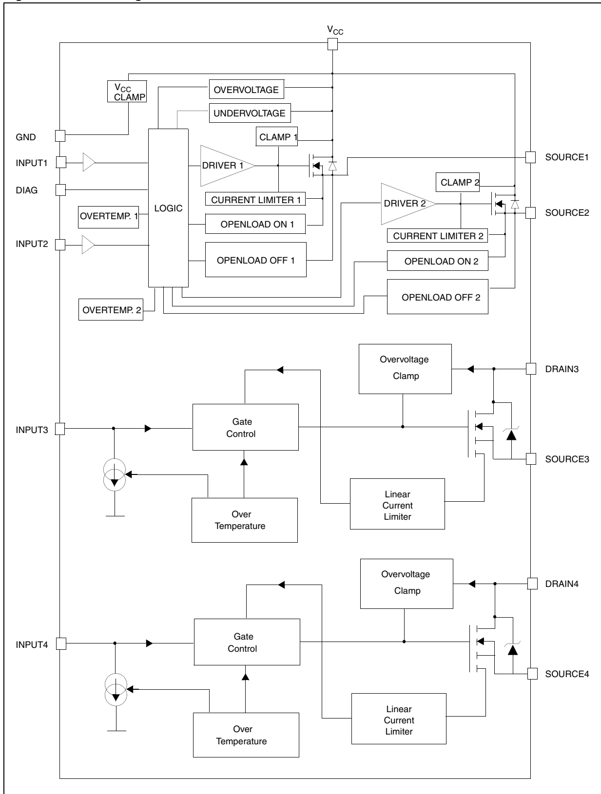
Figure 2. Block diagram
